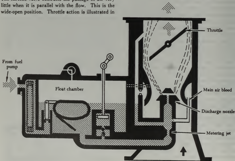
FIGURE 3-6. Fuel discharge.
